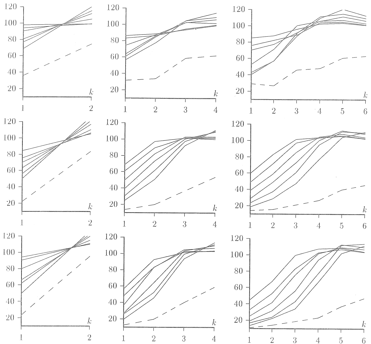
Figure 3: Query time using the index divided by query time using the on-line algorithm (percentage). The rows correspond to q = 3, 4 and 5 . The columns correspond to m = 8, 16 and 24 . The dashed line corresponds to character addressing, full lines to block addressing. From lower to upper (at k = 1 ) they correspond to b = 2, 4, 8, 16, 32 and 64 Kb.
